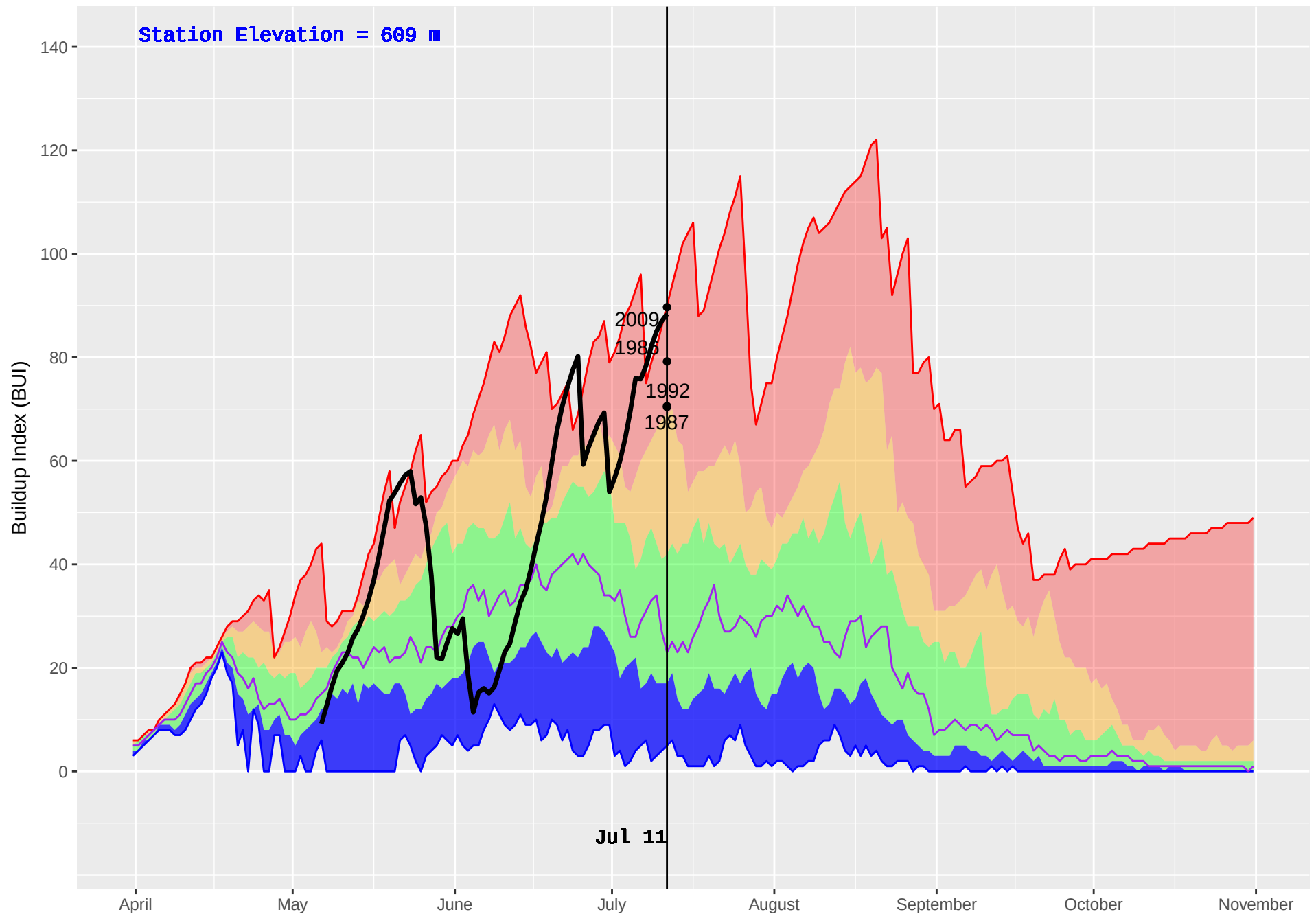
BOB QUINN LAKE (113) : Historical (1984–2016) and Current (2018) Noon Buildup Index (BUI)
